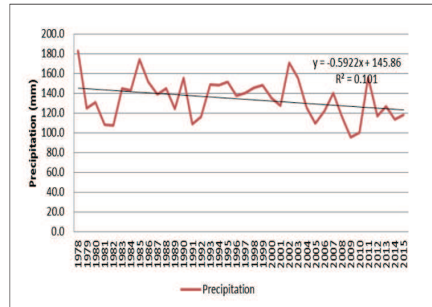
Figure 2. Precipitation trend of the Kathmandu Valley (1978-2015)
