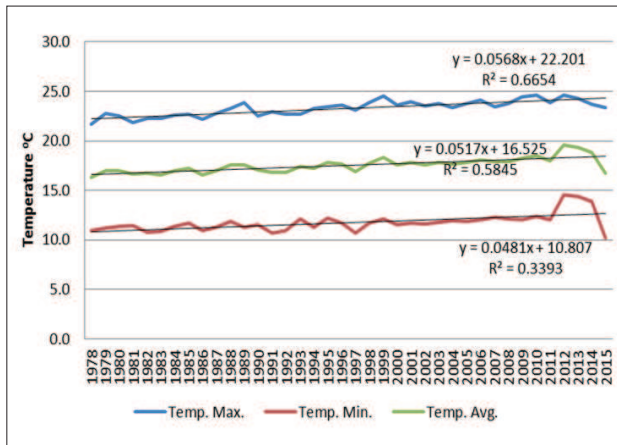
Figure 1. Temperature trend of the Kathmandu Valley (1978-2015)
